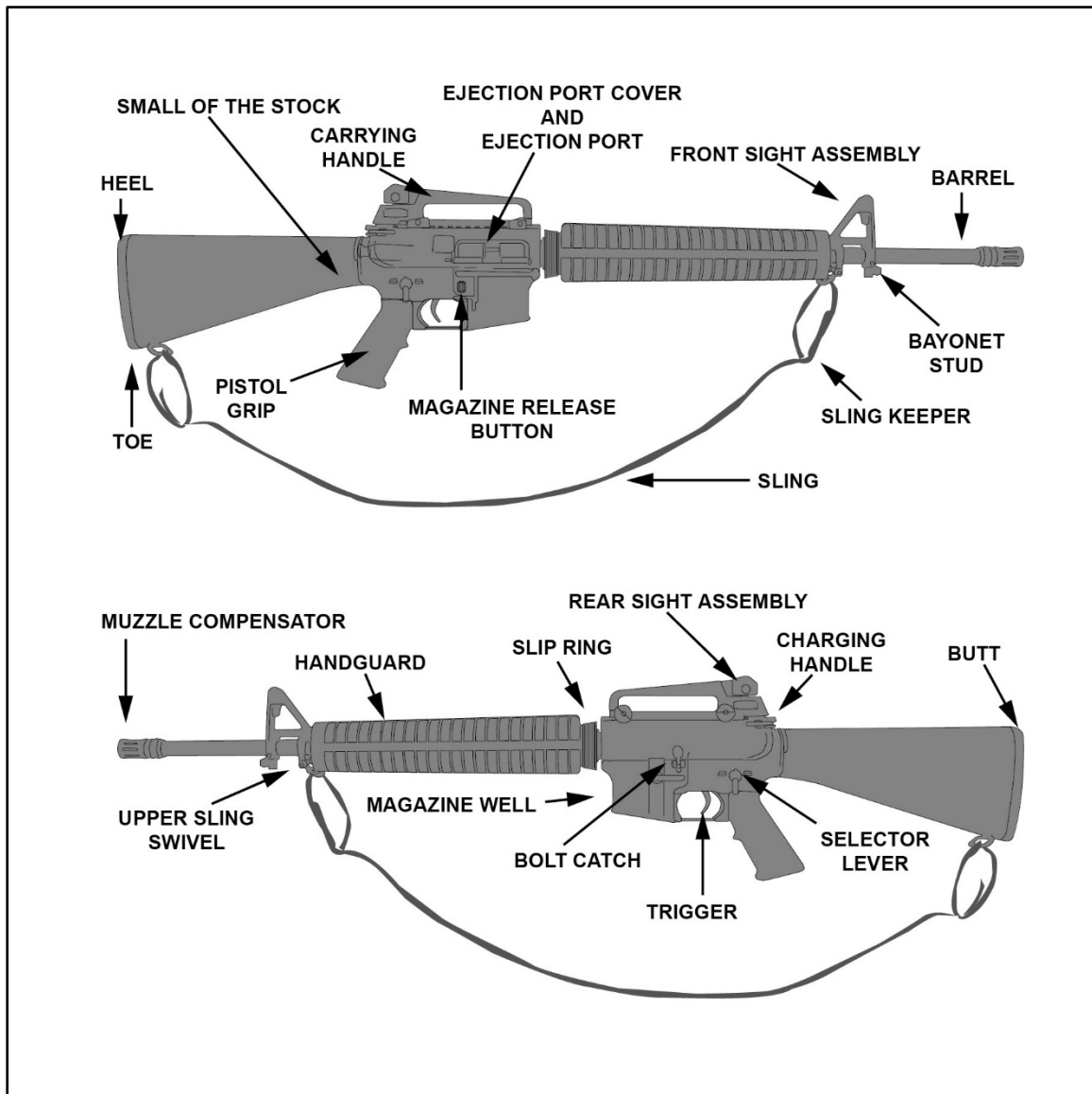
Figure B-1. Nomenclature, M16-series rifle
