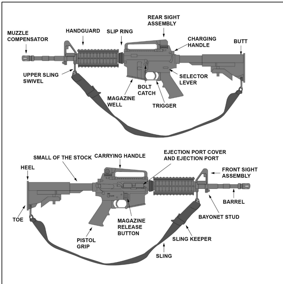
Figure 5-1. Nomenclature, M4-series carbine
