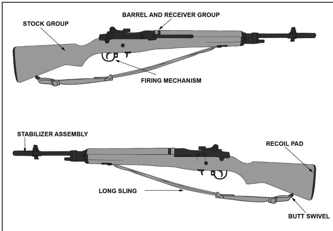
Figure C-1. Nomenclature, M14 rifle
