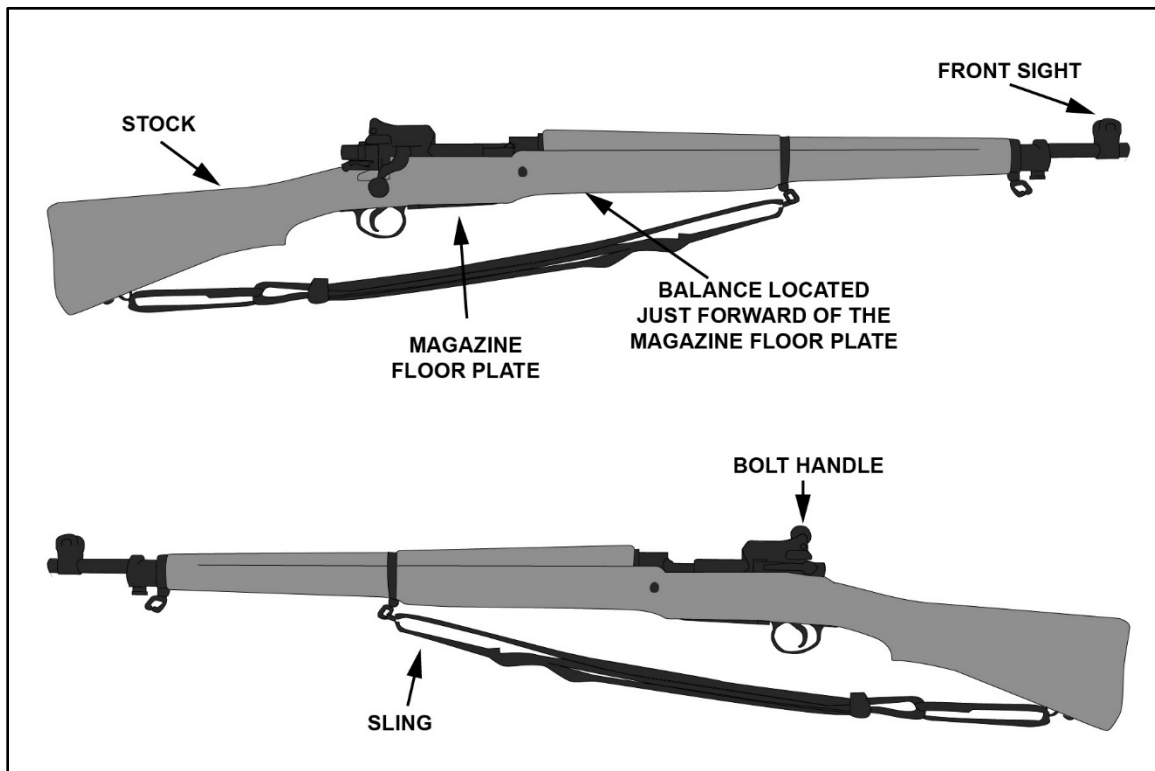
Figure D-1. Nomenclature, M1903 or M1917 rifle
